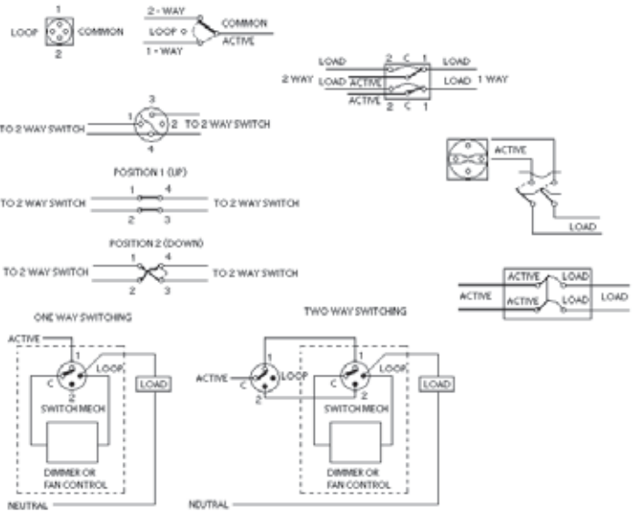
SINGLE POWER POINT SCHEMATIC WIRING DIAGRAM
